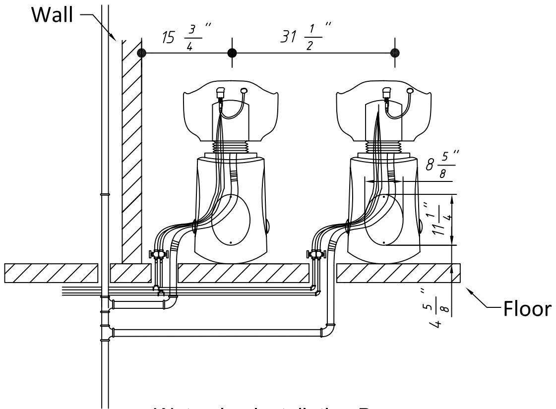
Water pipe installation B.
