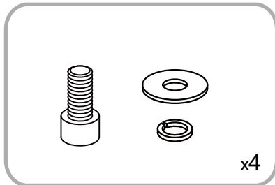
Screw ( M8X16MM) & Gasket
