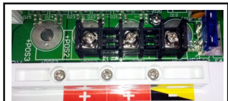
PCU 12V 10A & 20A models have ring terminal screw connectors as depicted above. N.B. the 10A model has only 2 outputs, all other models have 3 outputs.
