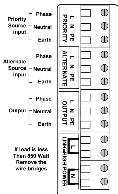
Wiring diagram
